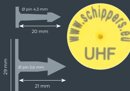
MS Tag Round UHF
