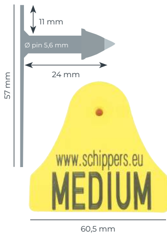
MS Tag Medium (Robust pin)
