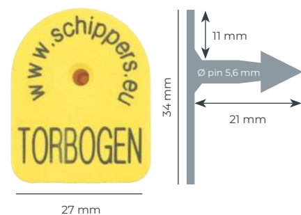
MS Tag Torbogen (Plastic pin)
