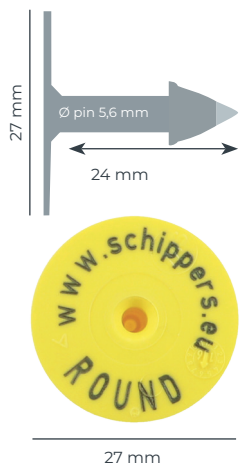
MS Tag Round (Robust pin)
