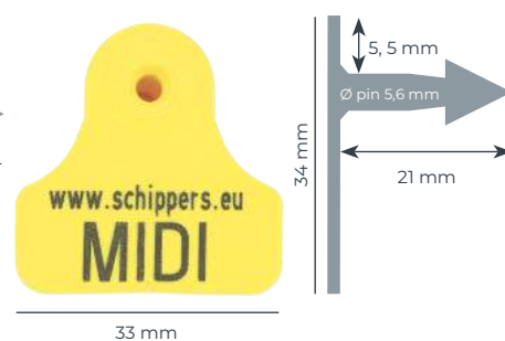
MS Tag Midi (Plastic pin)
