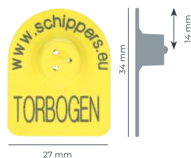
MS Tag Torbogen (Closed)
