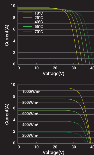
I-V Curve: (A-HCM340)
