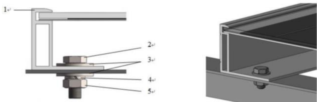
Figure 6 Schematic diagram1 of monofacial bodule with bolt Installation
