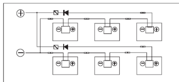
Parallel Connection
