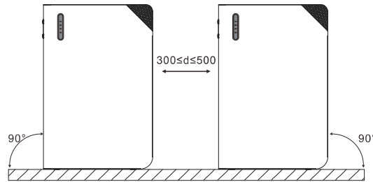
Ground(Two rows installtion)
