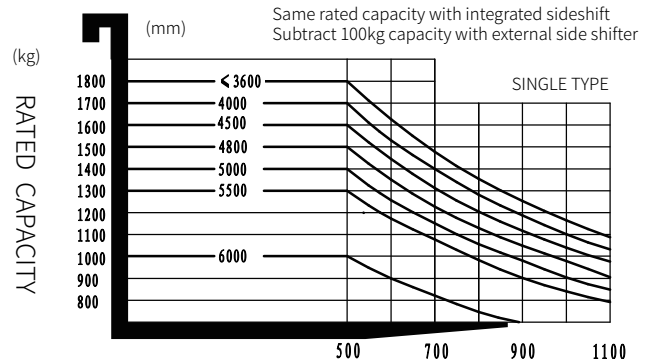
RATED CAPACITIES AND LOAD CENTERS GRAPH
