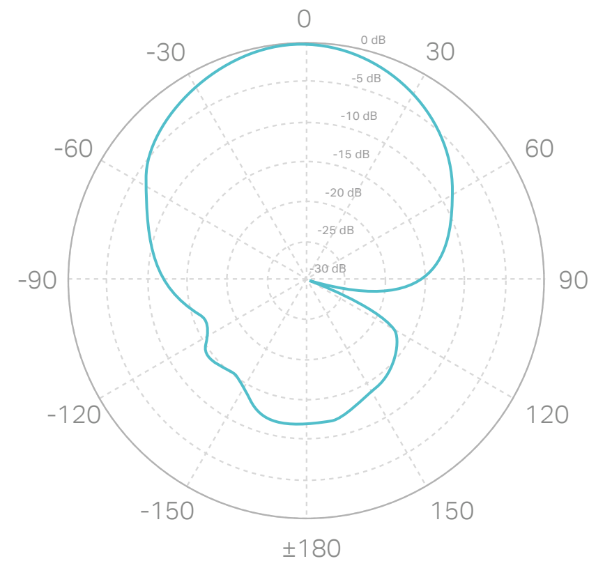
Vertical Azimuth
