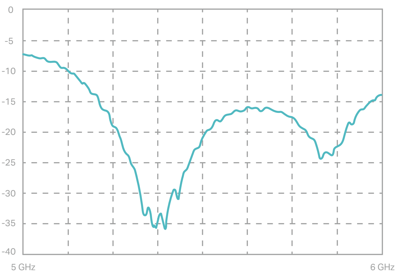
Return Loss
