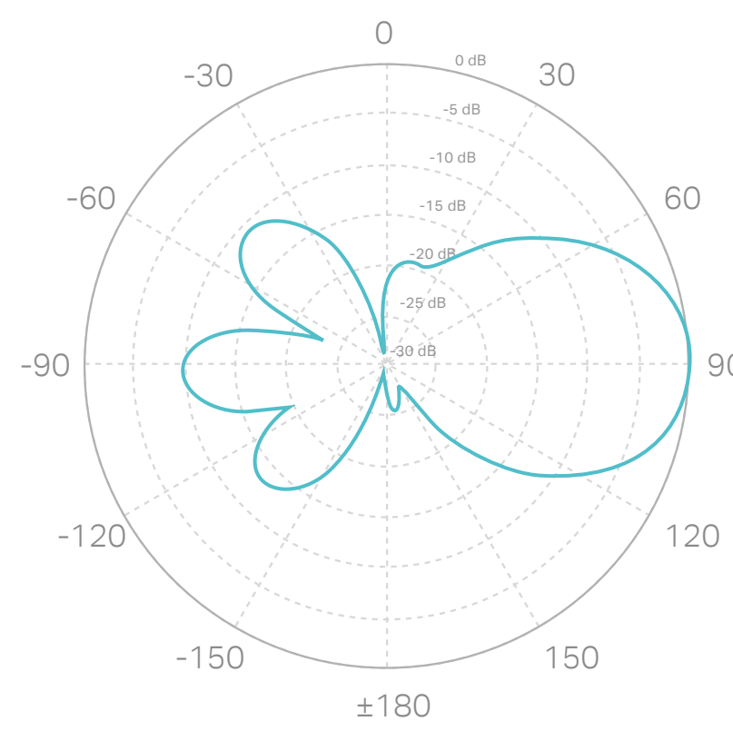
Vertical Elevation
