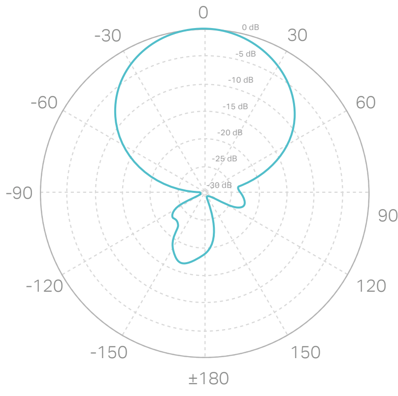
Horizontal Azimuth
