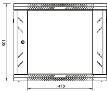
Front view (Toughened glass)
