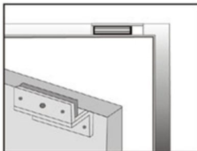
ZL Bracket Installation
