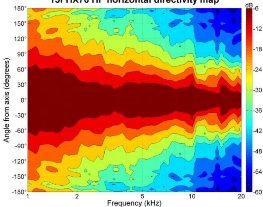
15FHX76 HF horizontal directivity map
