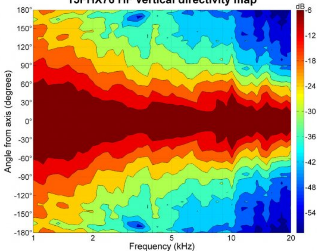
15FHX76 HF vertical directivity map
