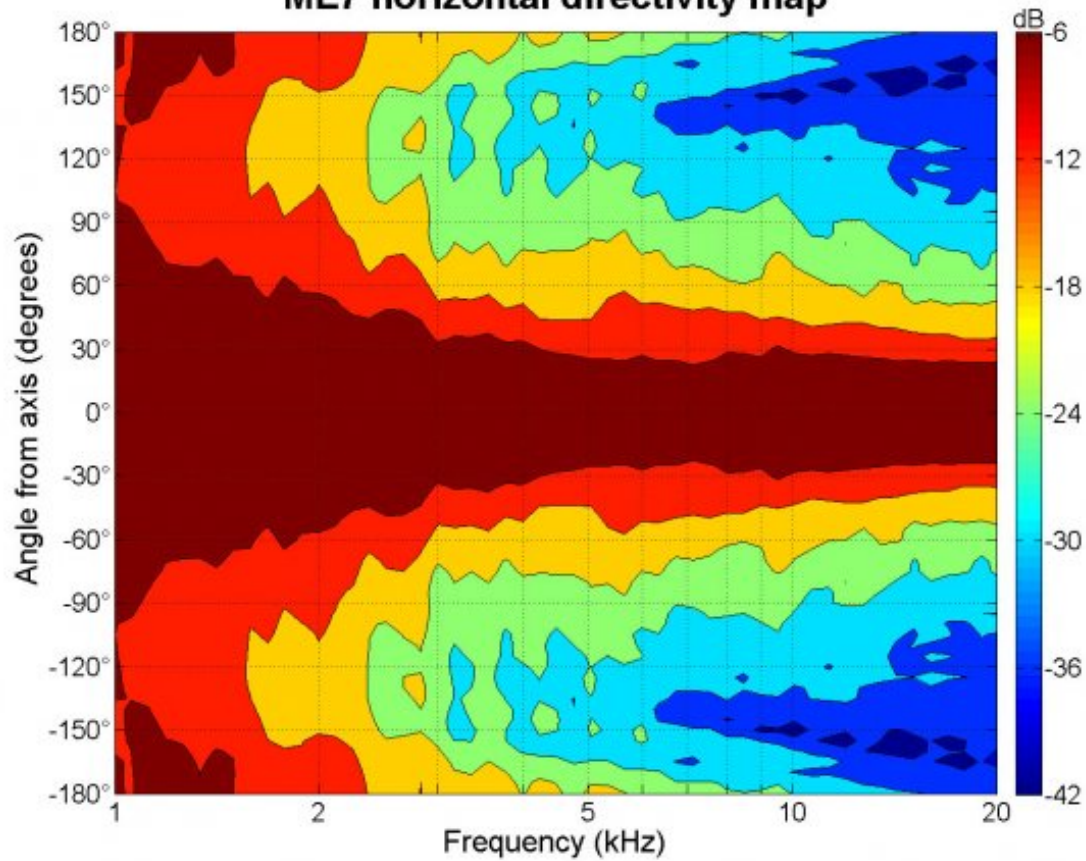
ME7 horizontal directivity map
