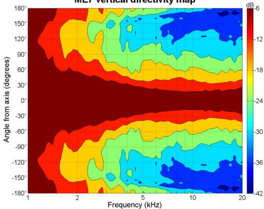
ME7 vertical directivity map
