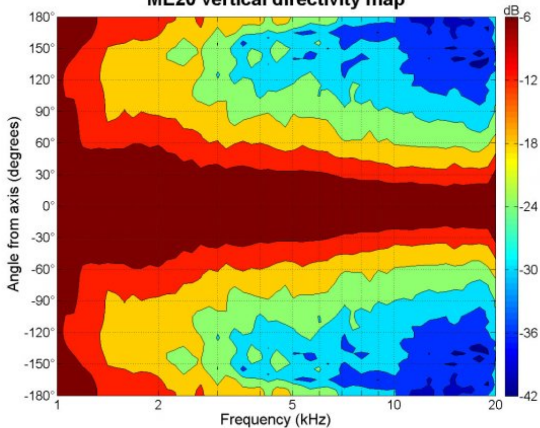
ME20 vertical directivity map
