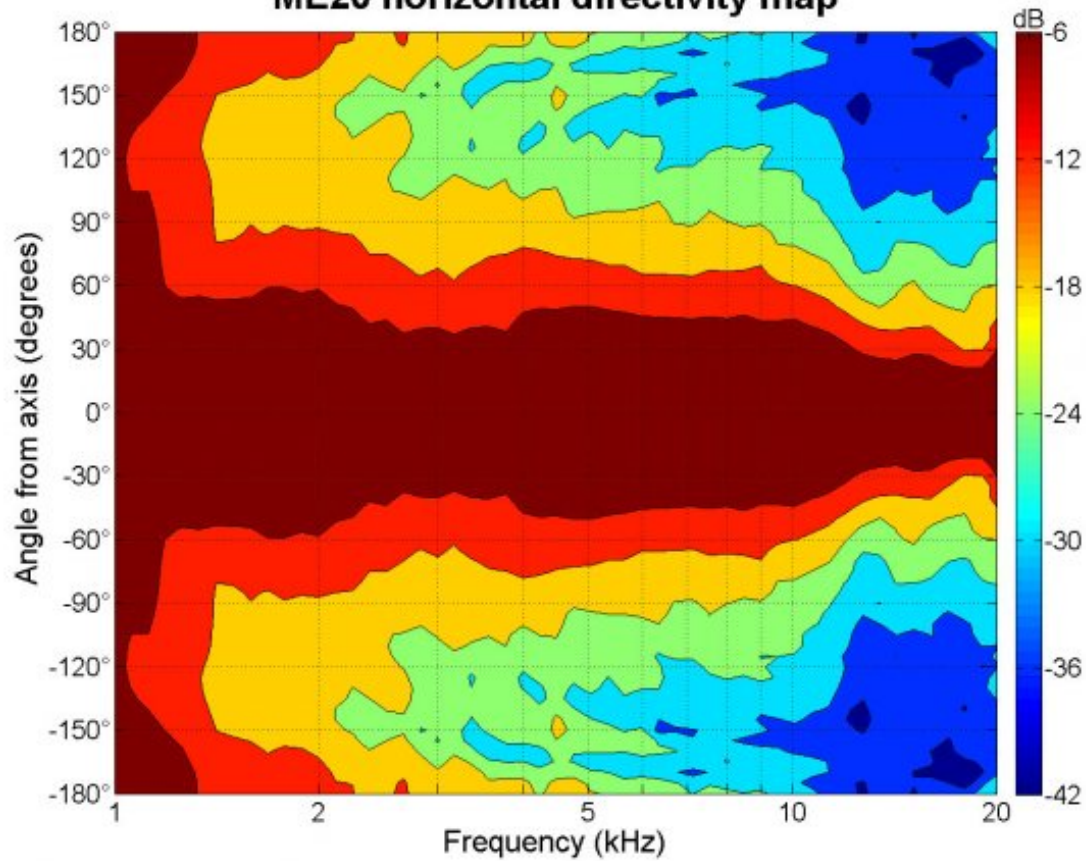
ME20 horizontal directivity map
