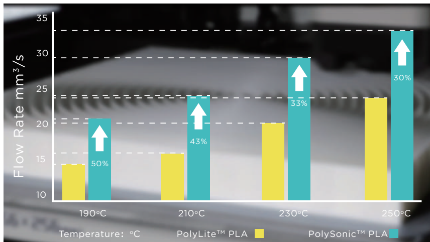
Fig.2 Comparison of the max flow rate of PolyLite™ PLA and PolySonic™ PLA with incremental temperatures (The reference extrusion testing is performed on a customized extrusion platform equipped E3D volcano hotend and 0.4mm nozzle with Hemera XS extruder.
