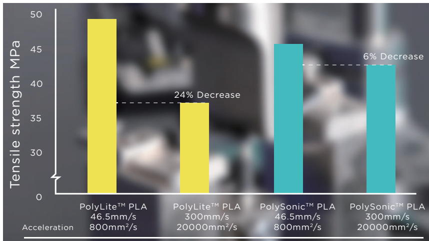
Fig.4 Comparison of tensile strength of PolySonic™ PLA and PolyLite™ PLA at high speed and classic speeds.
