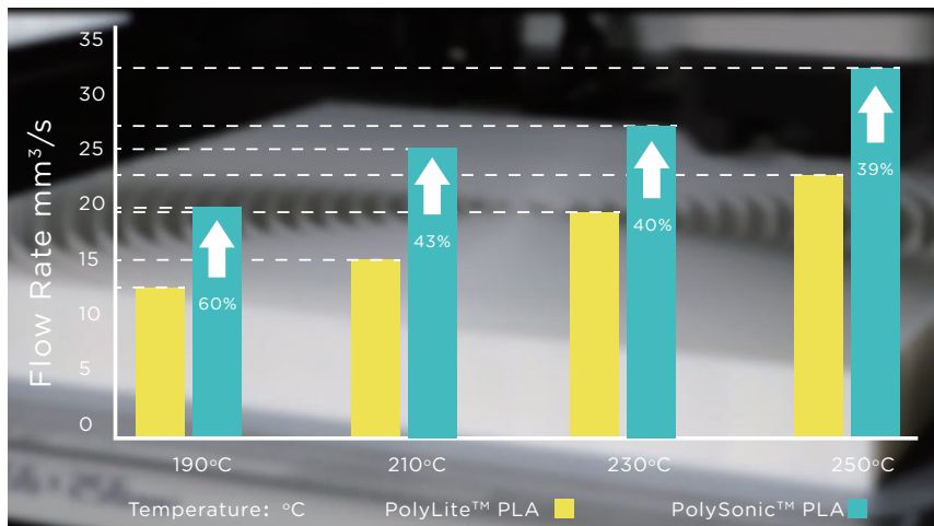
Fig.2 Comparison of the max flow rate of PolyLite™ PLA Pro and PolySonic™ PLA Pro with incremental temperatures (The reference extrusion testing is performed on a customized extrusion platform equipped E3D volcano hotend and 0.4mm nozzle with Hemera XS extruder).
