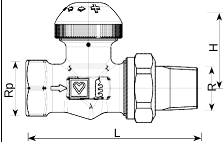
Cap termostatic Classic - 1 7260 06
