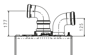
CONDUCTE DIVIZATE Ø80-80 mm
