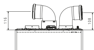
TWIN FLUE Ø80-80 mm
