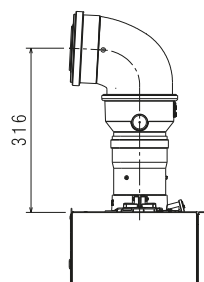
CONCENTRIC FLUE Ø80-125 mm
