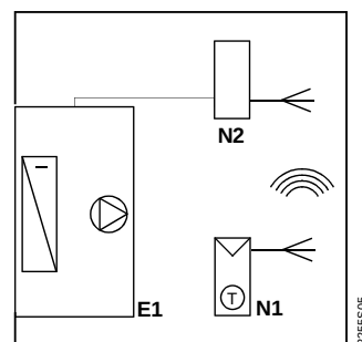
Cooling unit
