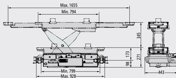
J40PY
