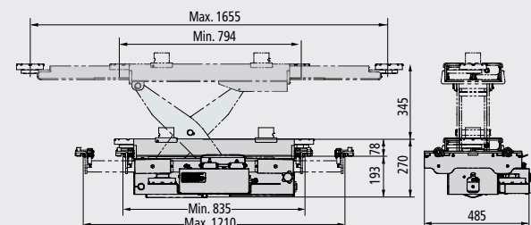
J40PKL
