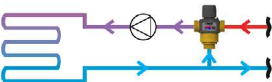
Floor heating
