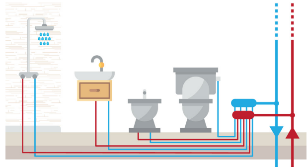
Figure 3 Manifold system.
