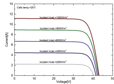
I-V Curves of SPP390QHFS at different irradiance
