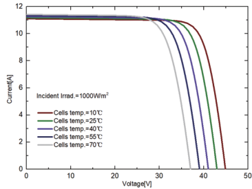
I-V Curves of SPP390QHFS at different cell temperature
