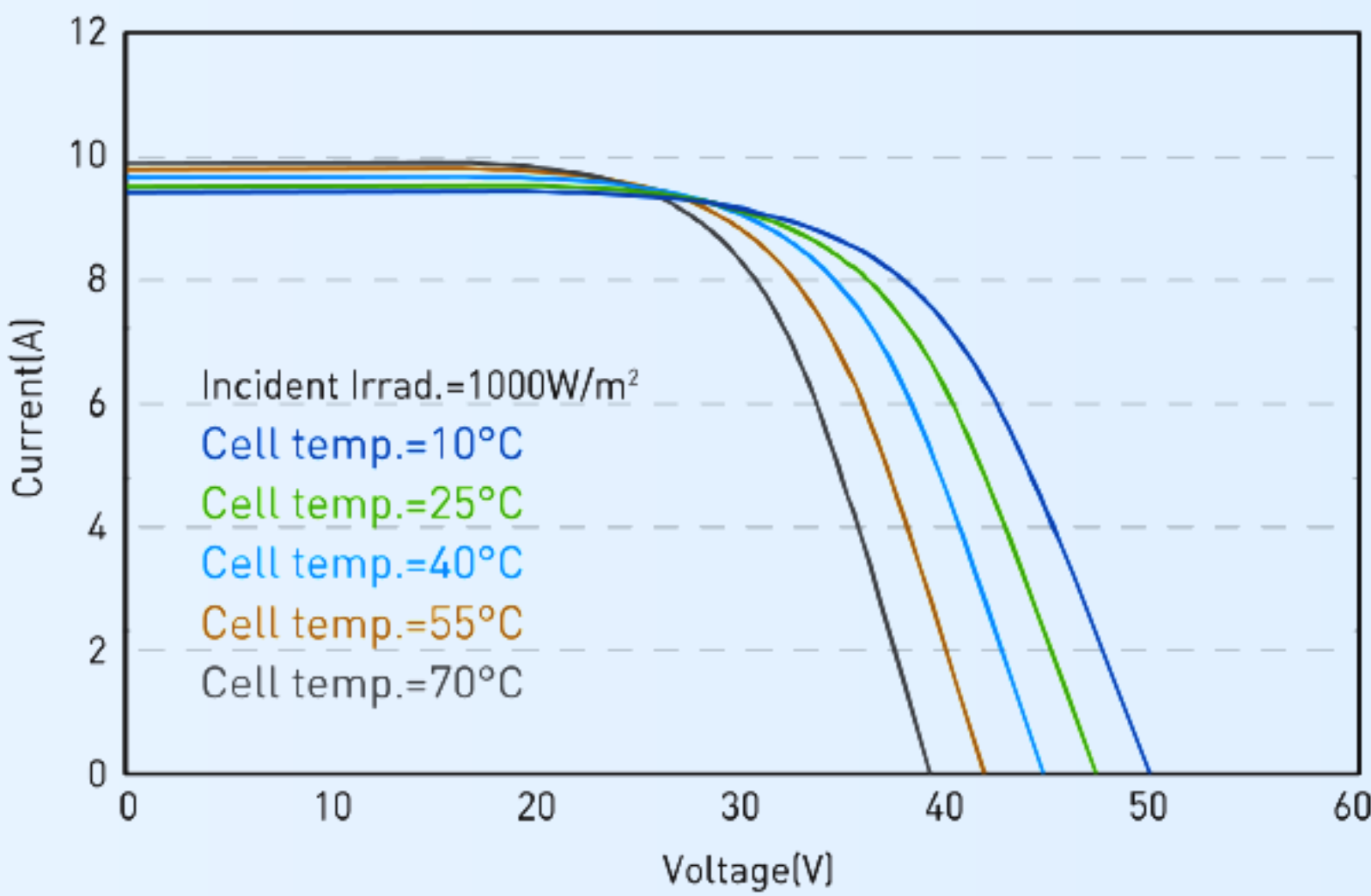
I-V Curve at Different Temperature [365W]
