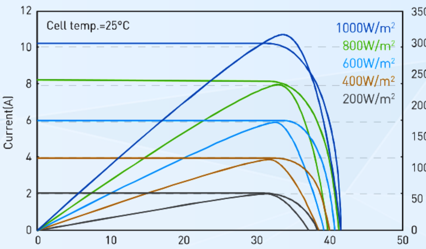
I-V/P-V Curve at Different Irradiation [365W]
