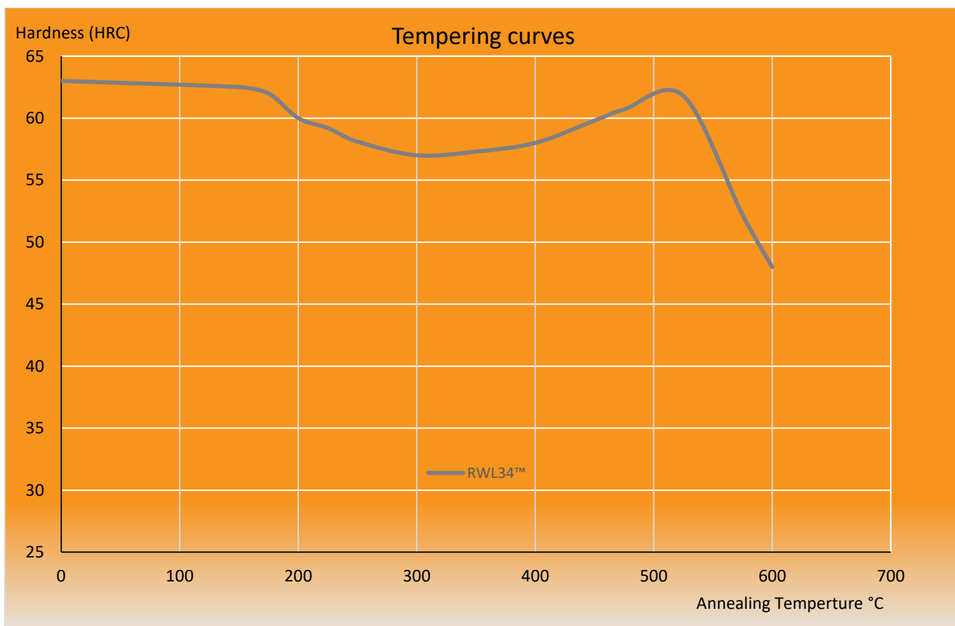
Diagram 2. Annealing temperature for RWL34™ ,austenitizing temperature 1080°C (1976F).
