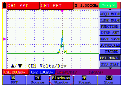
Figure 56: Blackman window
