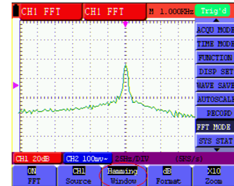
Figure 58: Hamming window
