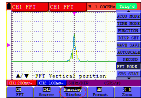
Figure 57: Hanning window
