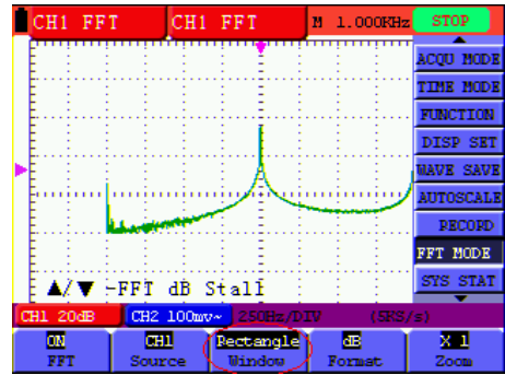
Figure 55: Rectangle window
