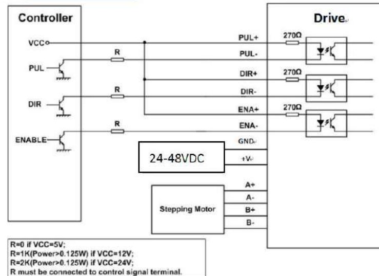
Figure 9: Typical connection
