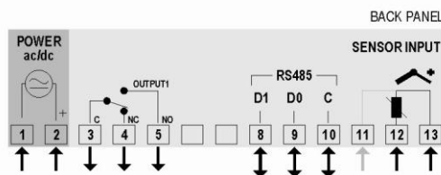
Fig. 1 – N321 terminals
