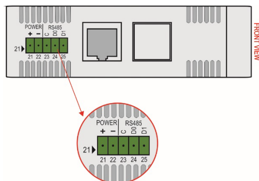
Figure 11 – RS485 connection
