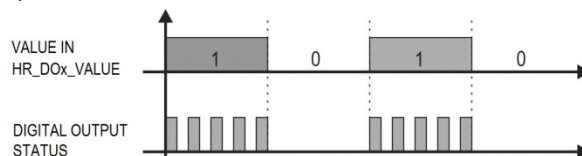
Figure 22 – "Pulse Train" mode
