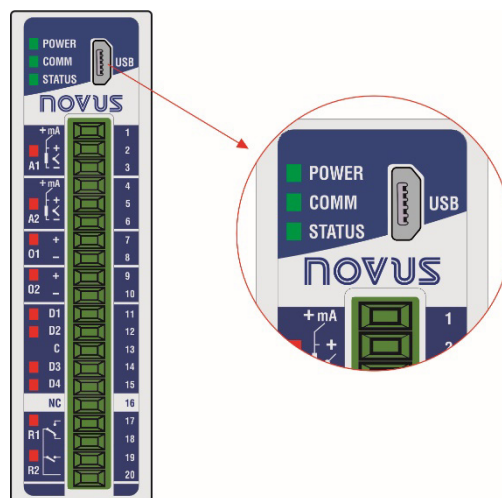
Figure 10 – USB connection
