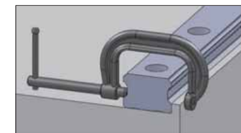
Fig1.8.13 Mounting the master Linear Guide rail
