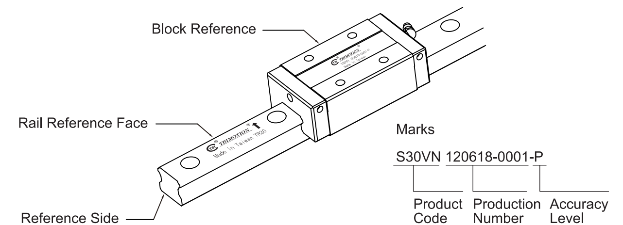
Fig1.8.1 Datum representation
