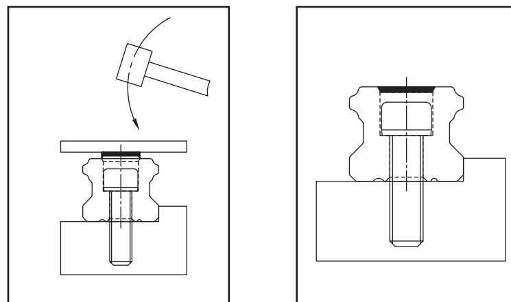
Fig2.13.2 Dustproof Rails
