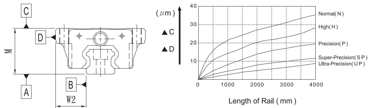
Fig2.10.1 Accuracy Standard
