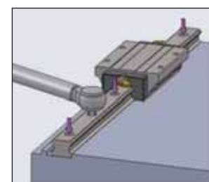
Fig1.8.10 Full Tightening of Mounting Bolts
