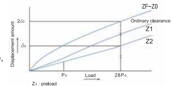
Fig1.10.2 Rigidity Data
