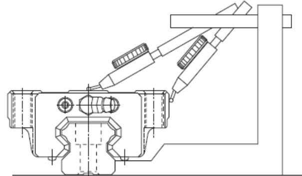
Fig1.11.1 Running parallelism
