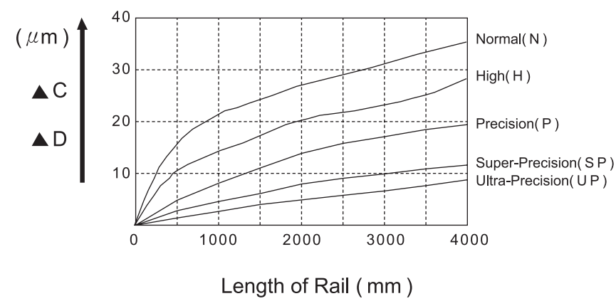
TR Rail Length and Running Accuracy.
