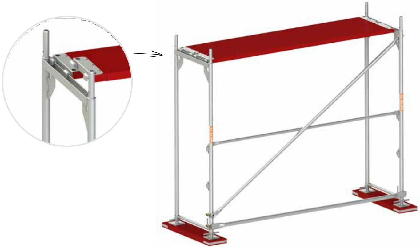
Fig. 5. First-storey base bay assembled.
