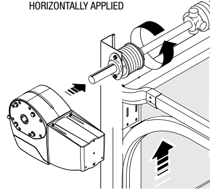
HORIZONTALLY APPLIED
