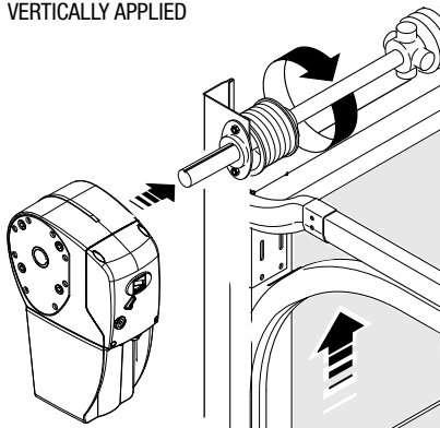
VERTICALLY APPLIED
