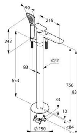
Dimensional drawing
