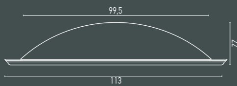
DM 504 ED: 113 cm ID: 99,5 cm D: 22 cm Fibre Reinforced Plastic (FRP)
