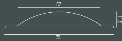
DM 503 ED: 75 cm ID: 57 cm D: 11,5 cm Polyurethane
