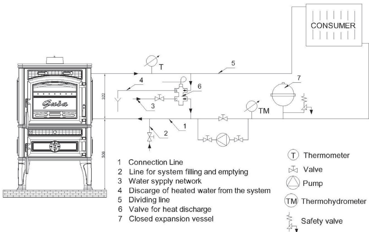
Picture.4 Scheme of closed system
