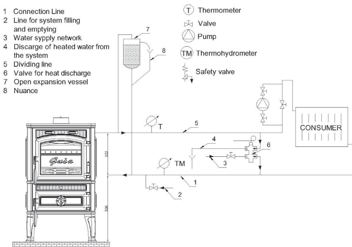
Picture.5 Scheme of open system
