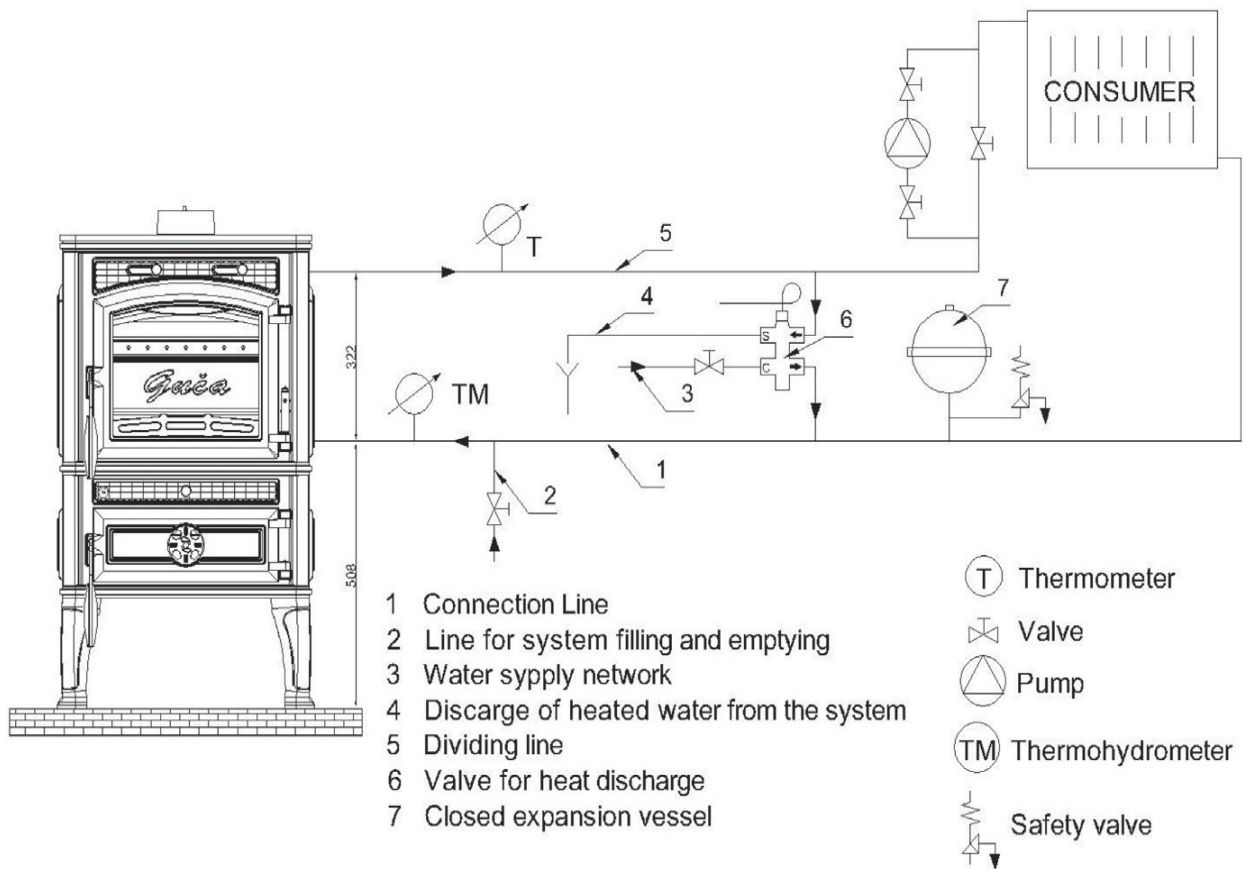
Picture.3 Scheme of closed system
