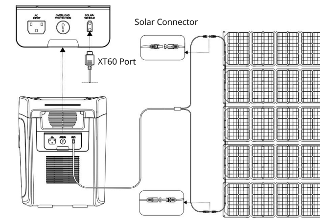
Figure I. 200W Solar Panels x 5
